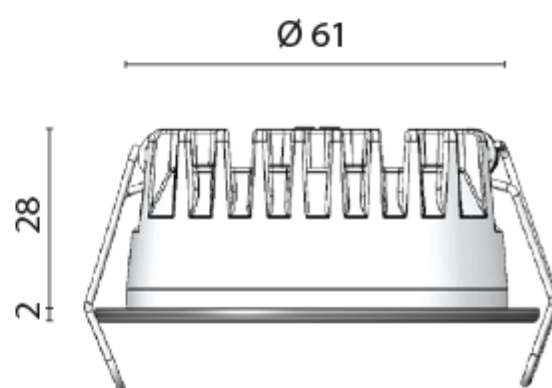
Power Led
